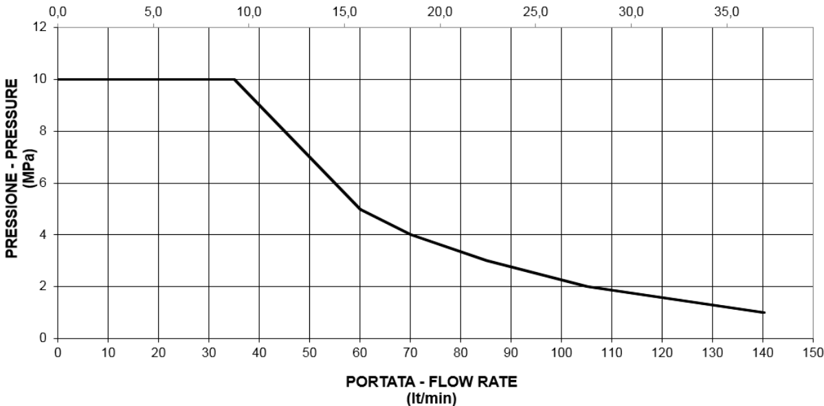
DIAGRAMMA PORTATA - PRESSIONE PRESSURE-FLOW RATE DIAGRAM
